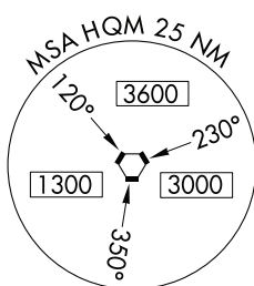
Multiple MSA's
