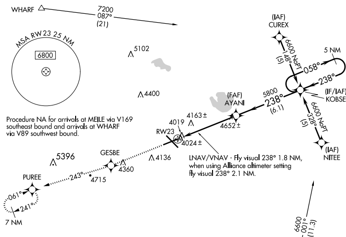
RNAV Approach
